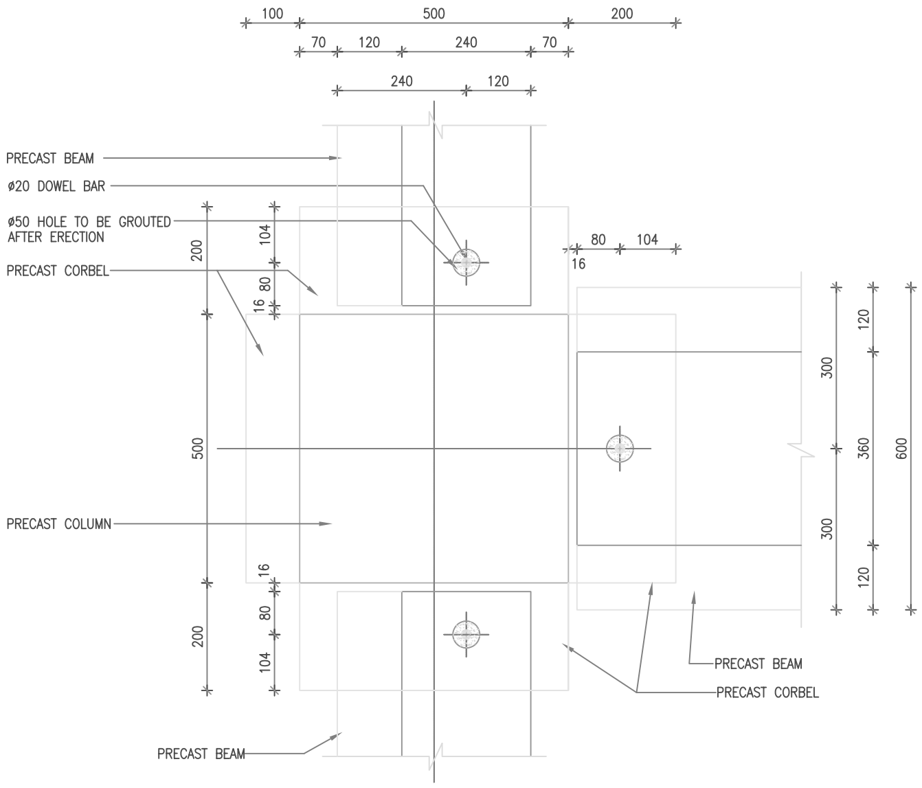
BEAM COLUMN ERECTION DETAIL
