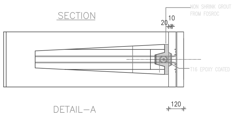
BOUNDARY WALL TYPE-2
