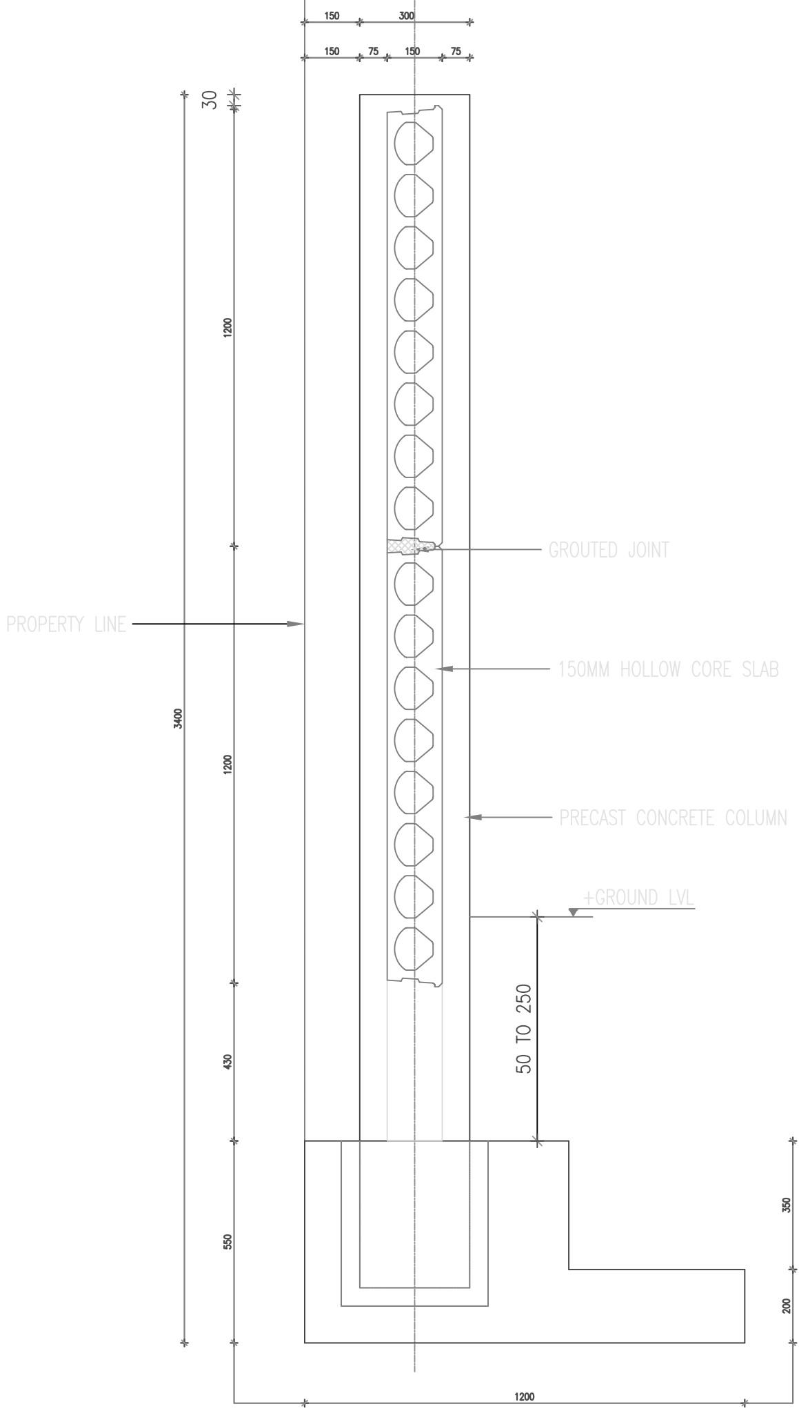
BOUNDARY WALL TYPE-3
